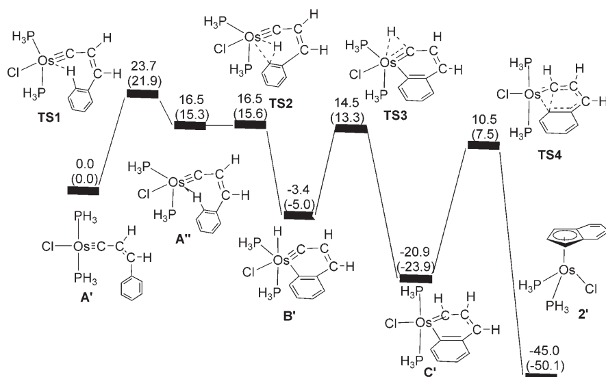
Figure 2. Energy profile for the formation of 2' from A' . The calculated relative free energies and reaction energies (in parentheses) are given in kcal mol -1 .
